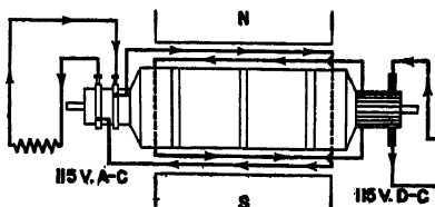
Dynamotor circuit.
